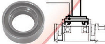
BEARING ATTACHMENT
